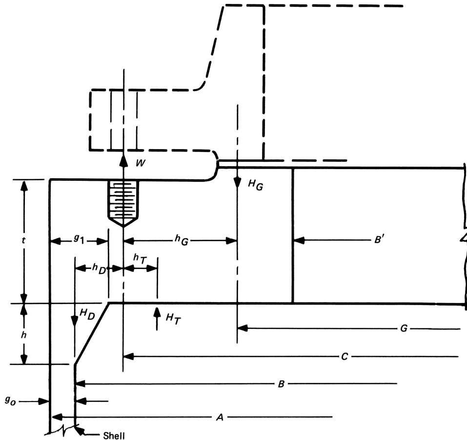
Figure XX-13.1 Reverse Flange
