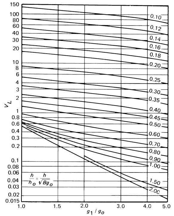
Figure XX-7.5 Values of V_L (Loose Hub Flange Factors)
