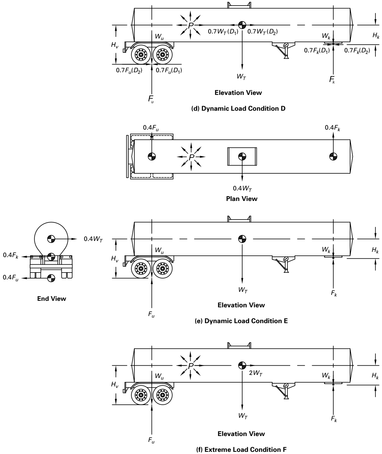
Figure 1-1.4 Loading Conditions (Cont'd)
