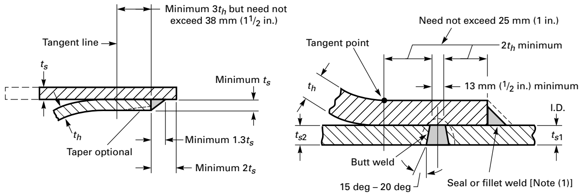
Figure TW-130.5-1 Heads Attached to Shells (See Table TW-130.4 for Limitations) (Cont'd)
