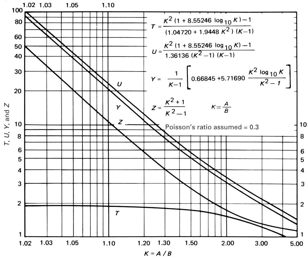
Figure XX-7.1 Values of T , U , Y , and Z (Terms Involving K )
