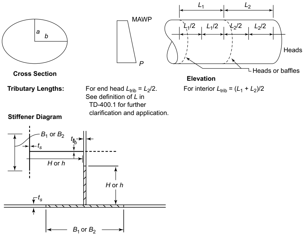
Figure VIII-2-3 Noncircular Cargo Tank Structural Properties
