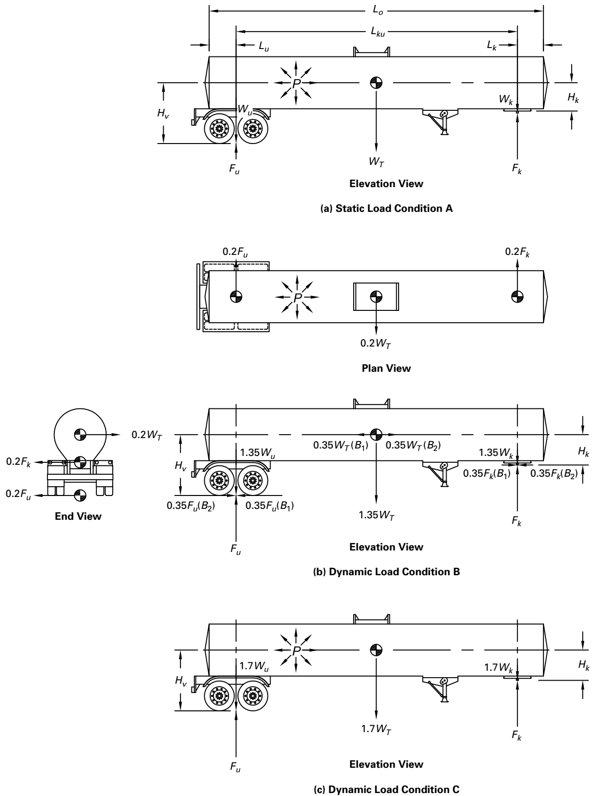
Figure 1-1.4 Loading Conditions
