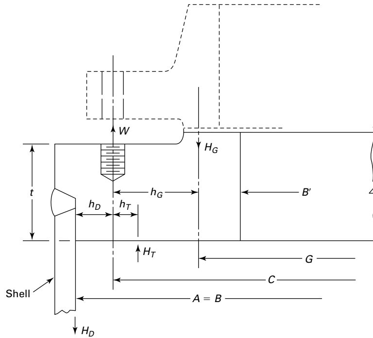
Figure XX-13.2 Loose Ring Type Reverse Flange
